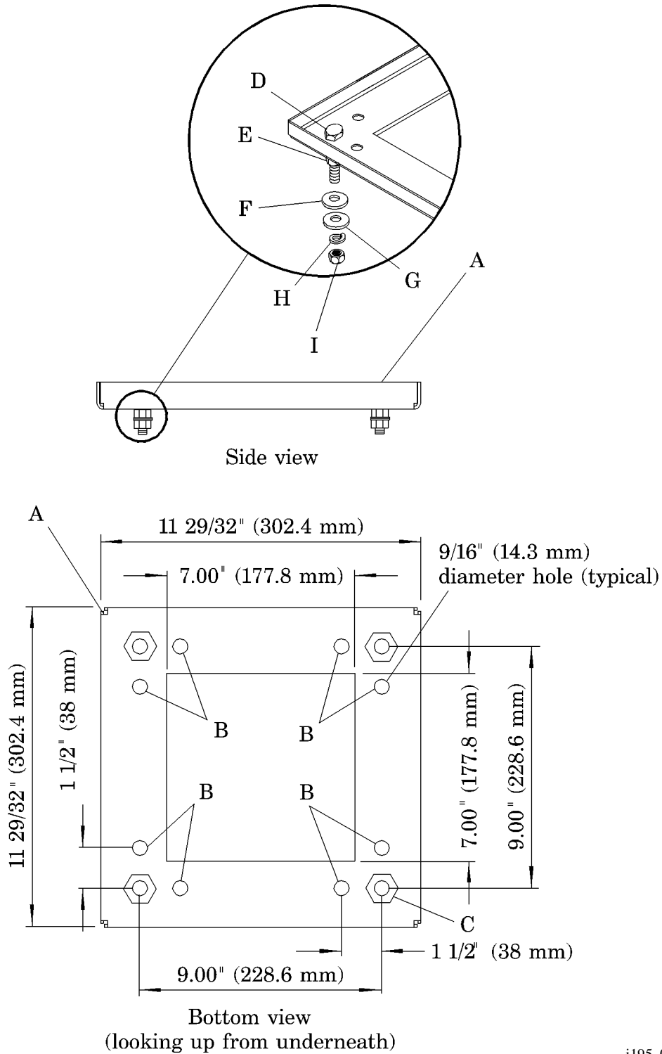
Figure 1. Ceiling Column Rough-In Set-ups Information
