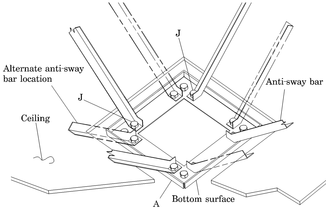
Figure 2. Ceiling Column Rough-In Installation
